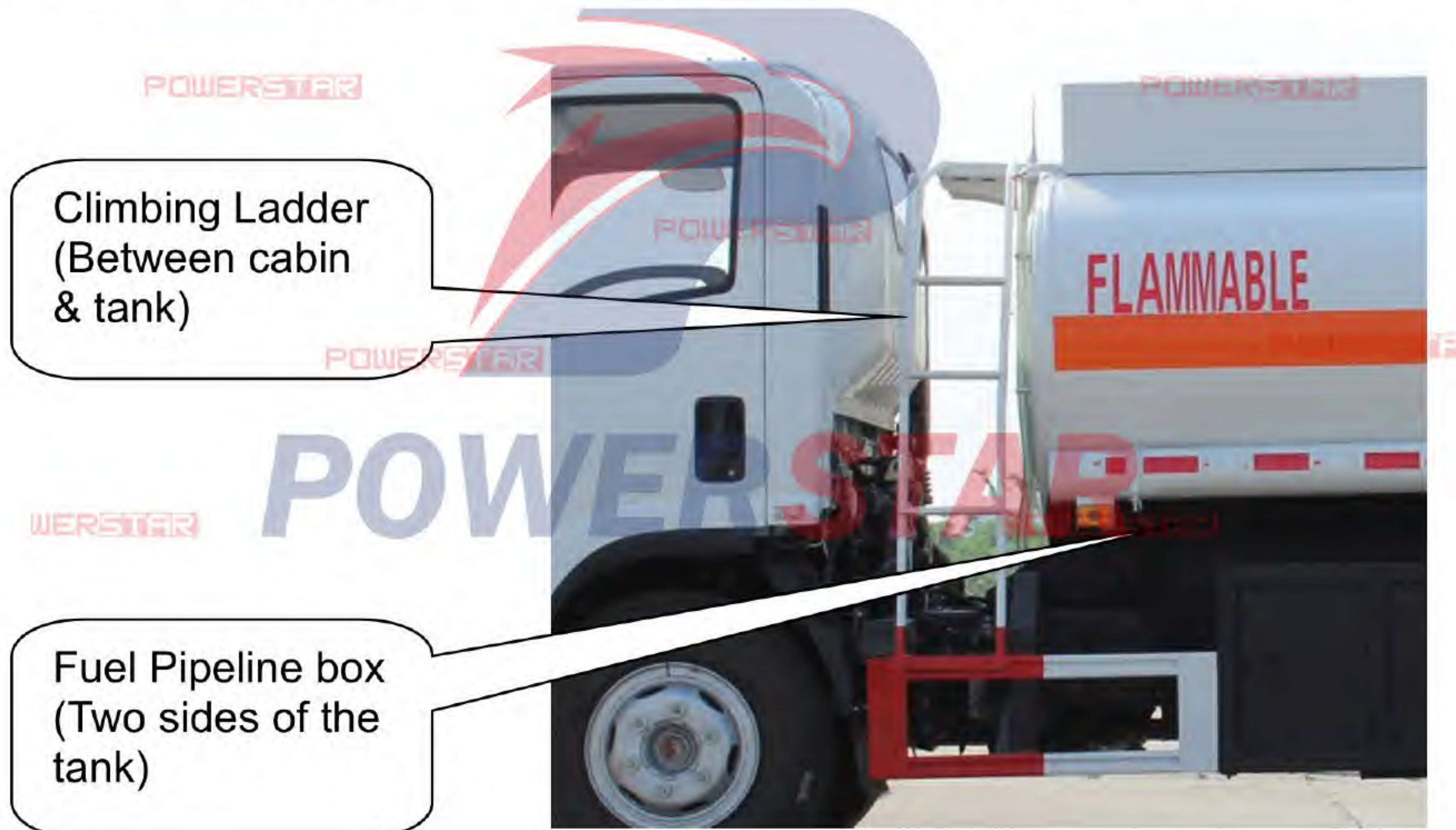
Side of the Tank: Climbing ladder with three level, Pipeline storage box & Fire-extinguisher storage box
